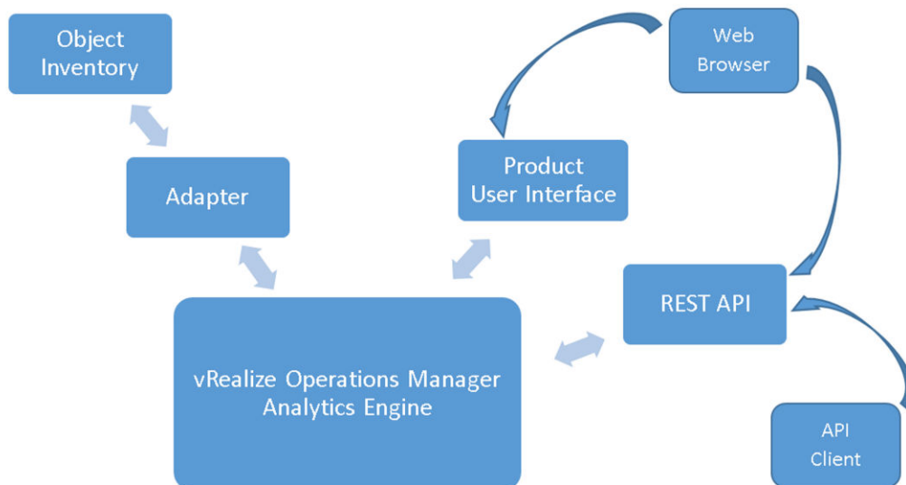
图 2-1 vRealize Operations Manager Simplified Architecture
