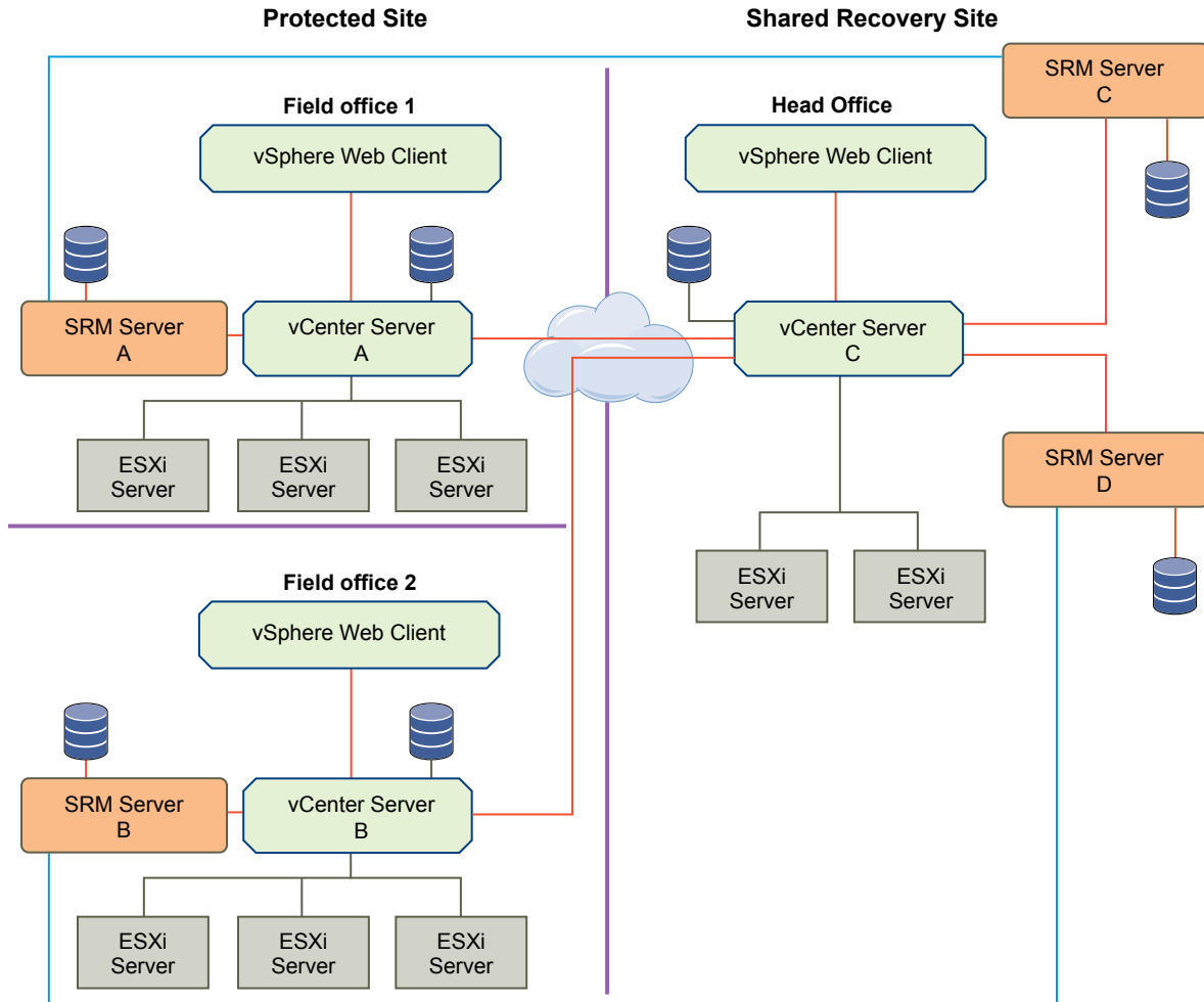
Figure 8-1. Example of Using Site Recovery Manager in a Shared Recovery Site Configuration
