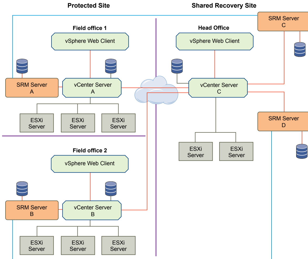
Figure 10-1. Example of Using Site Recovery Manager in a Shared Recovery Site Configuration
