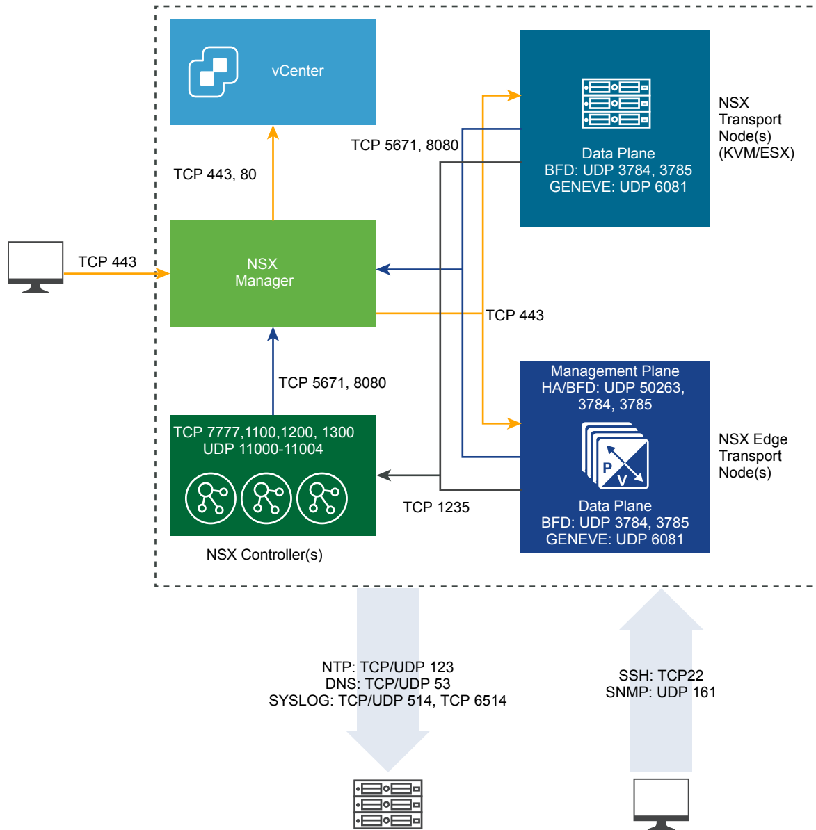
Figure 2-1. NSX-T Ports and Protocols
