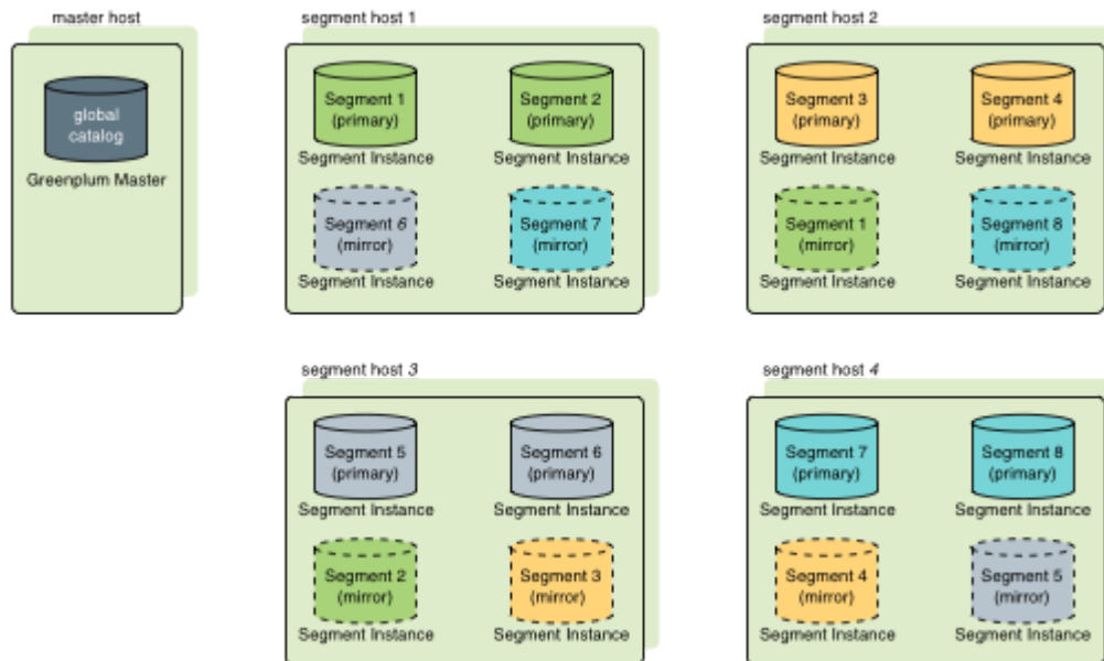
Figure 1 shows how table data is distributed across segments when spread mirroring is configured.
