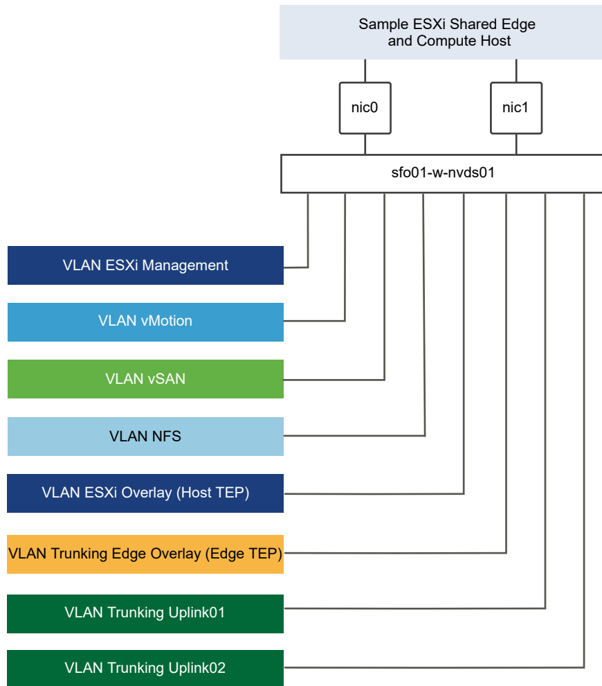
Figure 3-4. Virtual Switch Design for ESXi Hosts in the Shared Edge and Compute Cluster
