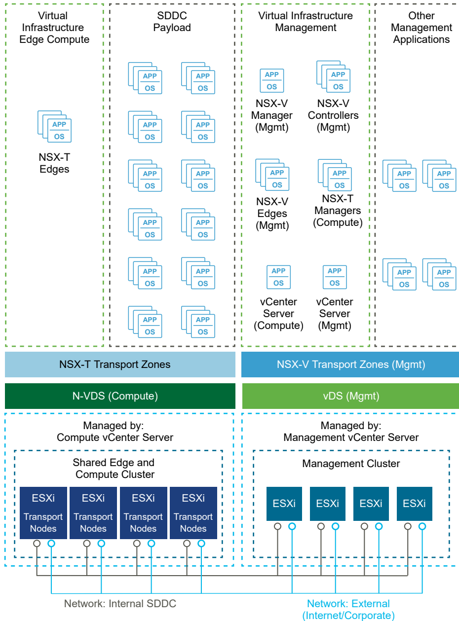
Figure 2-4. SDDC Logical Design
