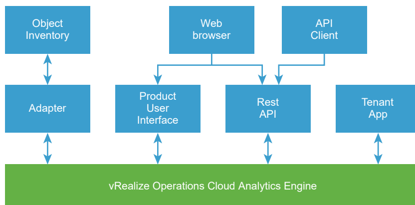
Figure 2-1. vRealize Operations Cloud Simplified Architecture
