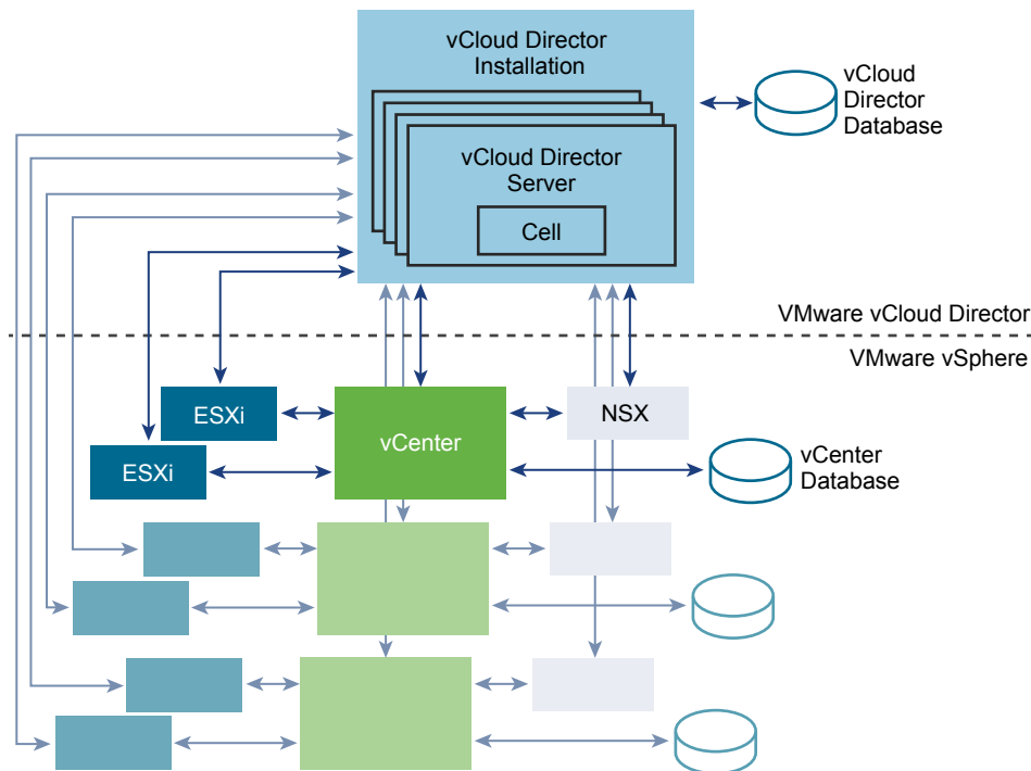
Figure 3-1. vCloud Director Architecture Diagram
