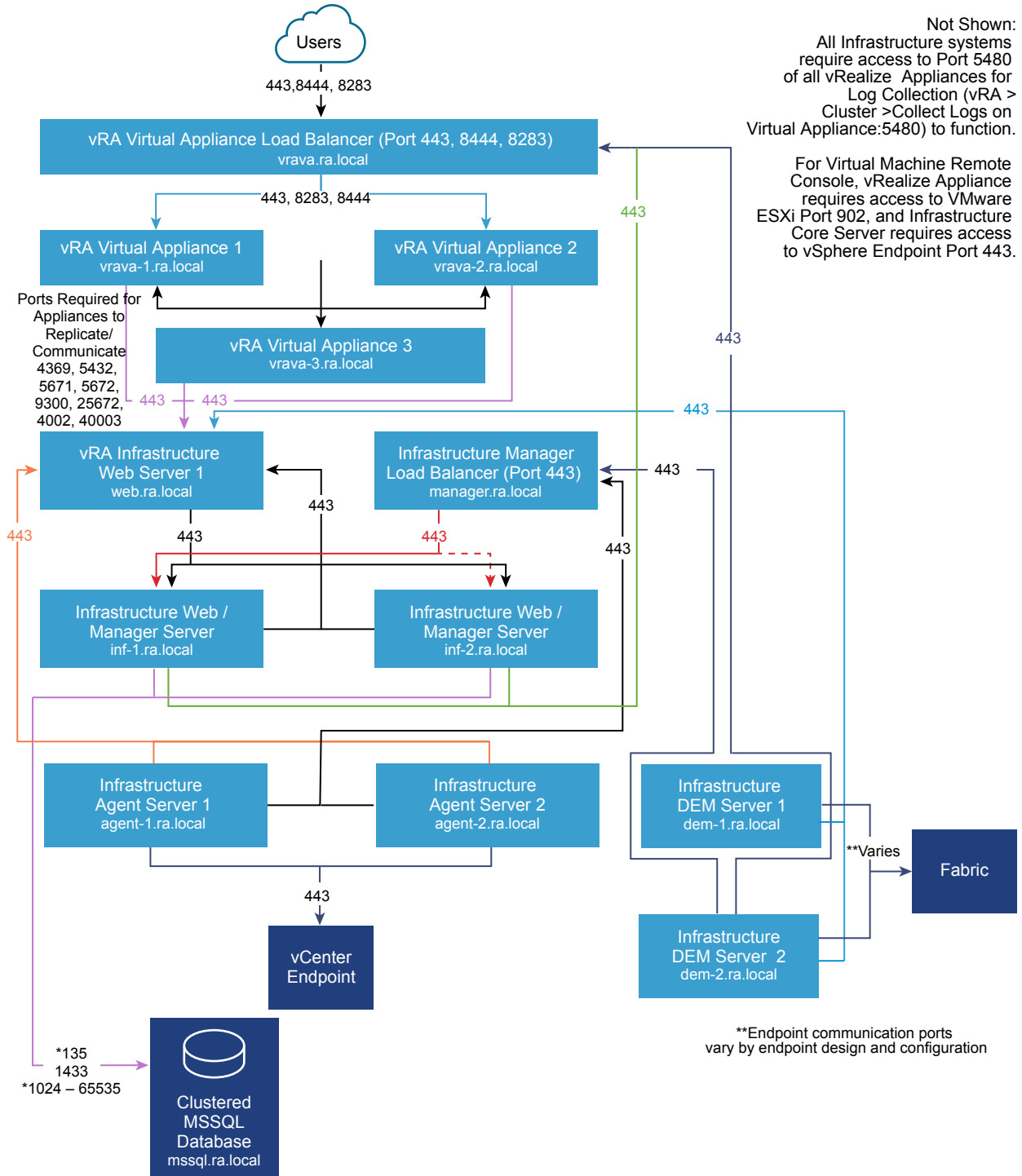
Figure 10-1. Minimum footprint for vRealize Automation medium configuration
