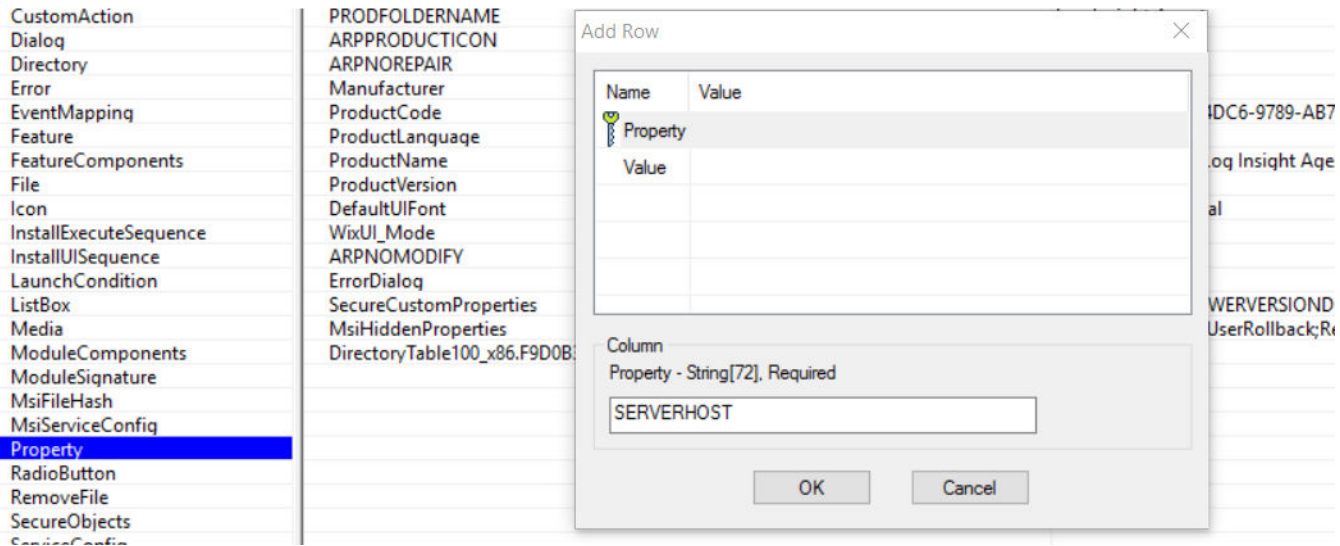
Figure 3-1. Property Table
