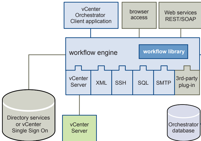
Figure 1-1. VMware vCenter Orchestrator Architecture
