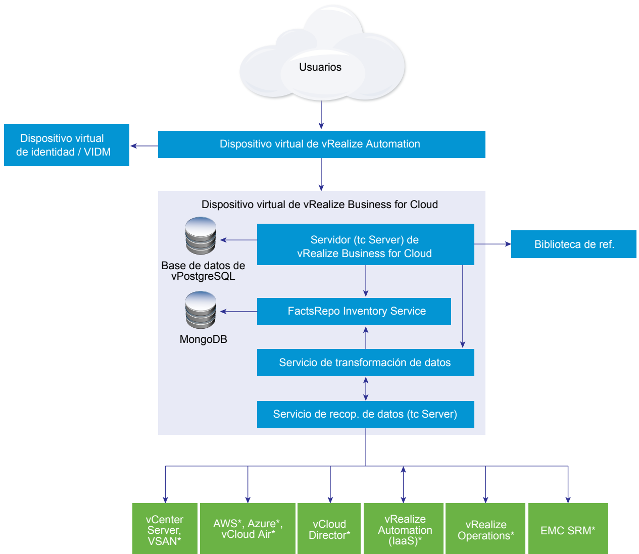
Figura 1-1. Arquitectura de vRealize Business for Cloud
