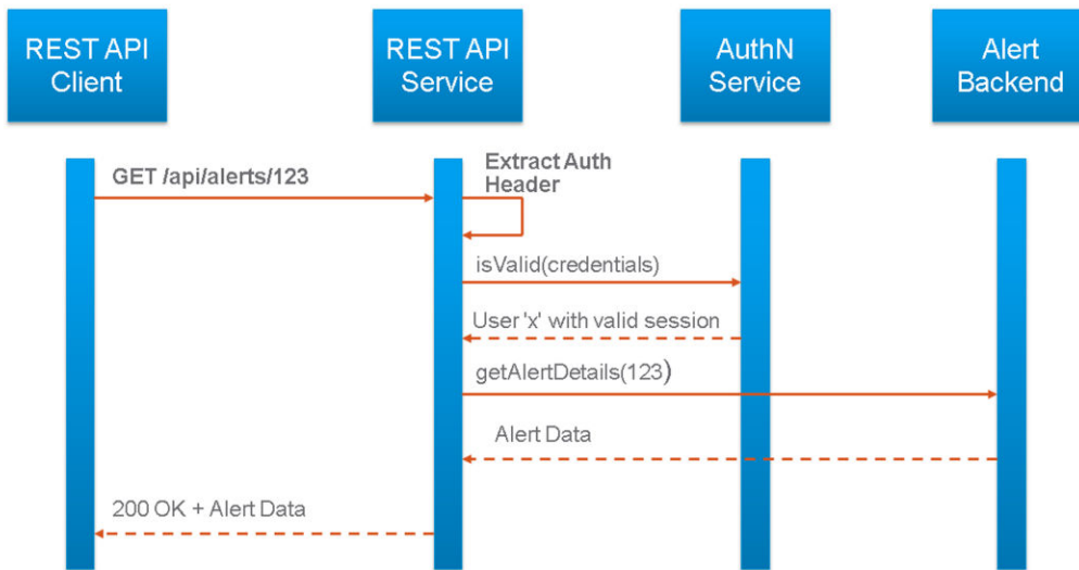
Figura 2-2. Scenario: Provide user credentials to obtain details about alert with ID 123
