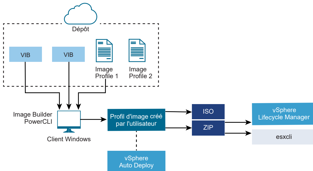
Figure 5-2. Architecture Image Builder
