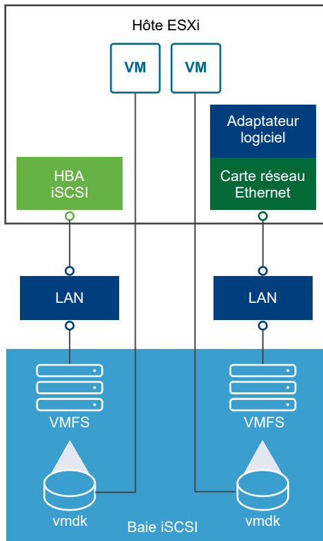
Figure 2-3. Stockage iSCSI
