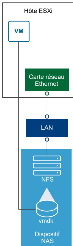
Figure 2-4. Stockage NFS
