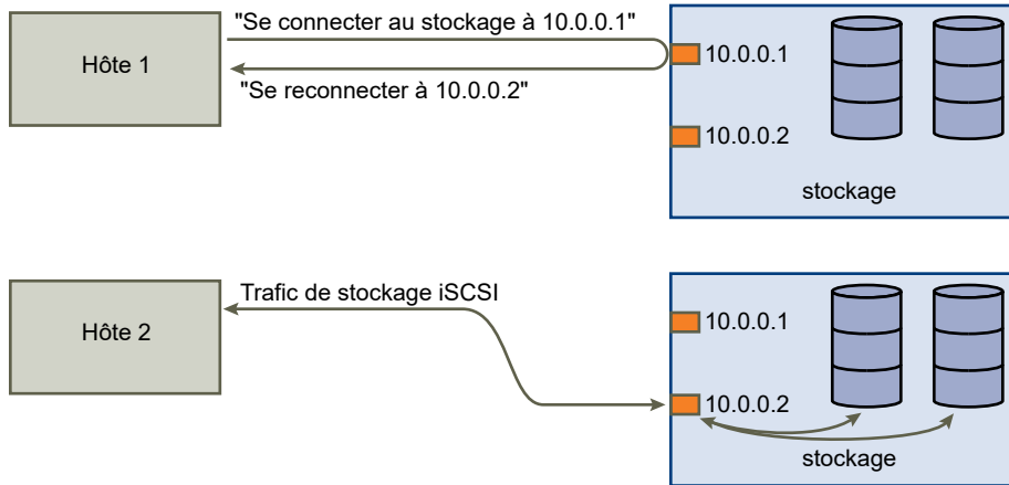
Figure 18-3. Redirection de port
