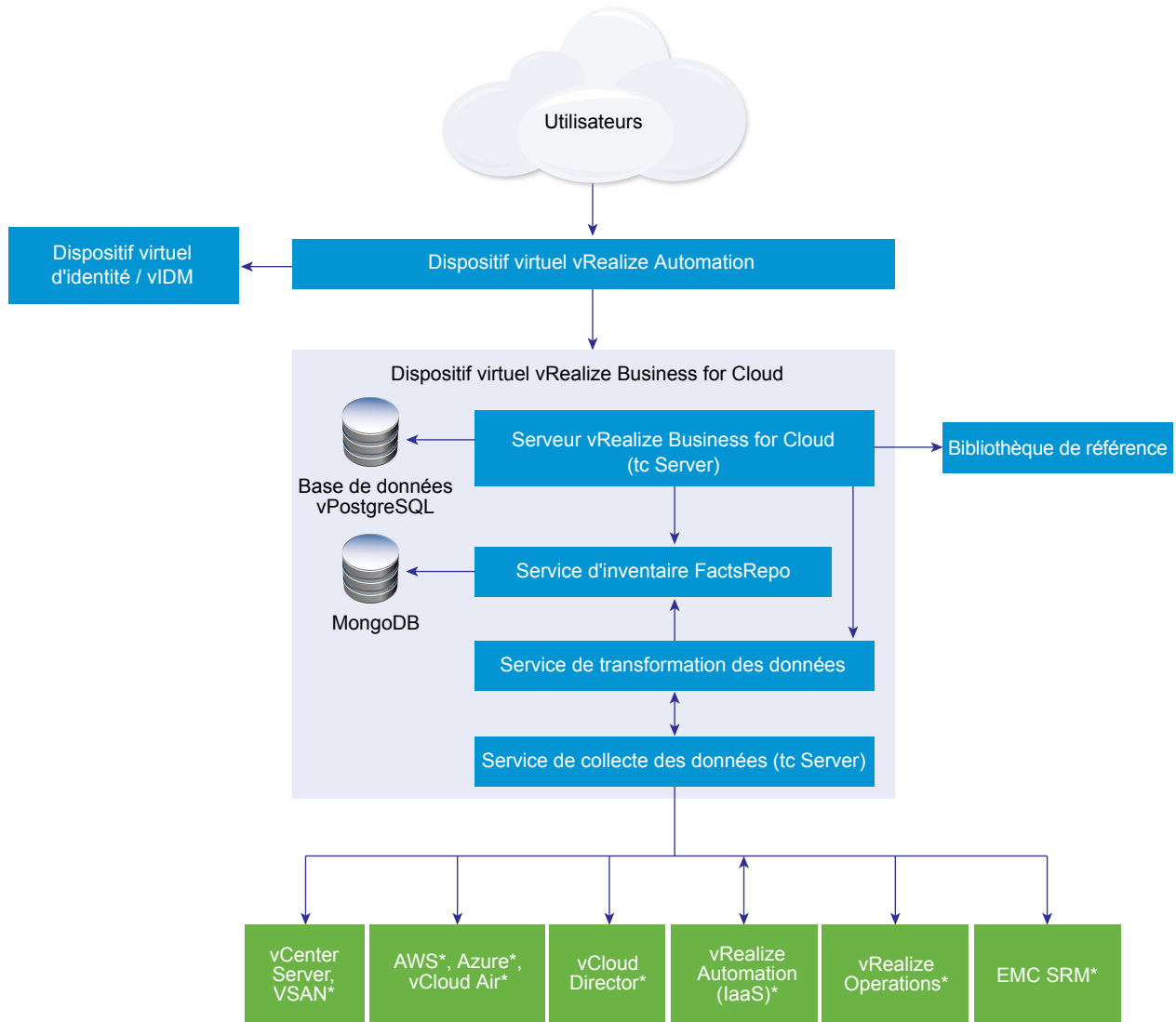
Figure 1-1. Architecture de vRealize Business for Cloud
