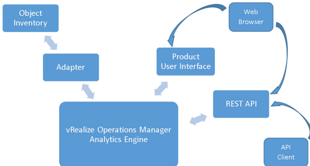
図 2-1. vRealize Operations Manager Simplified Architecture
